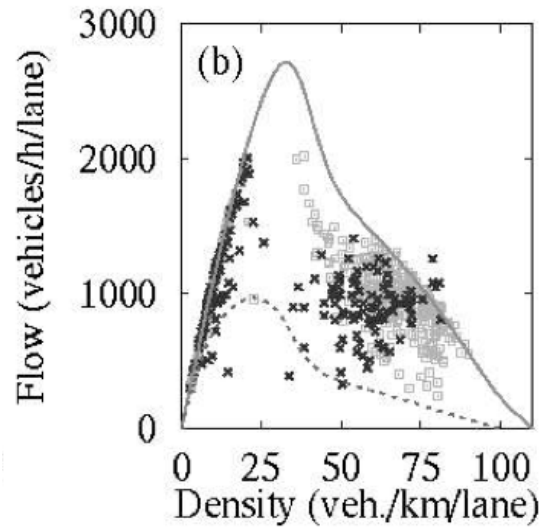
Figure 3. – Traffic Phase Diagram (D. Helbing, 2002 20 )
